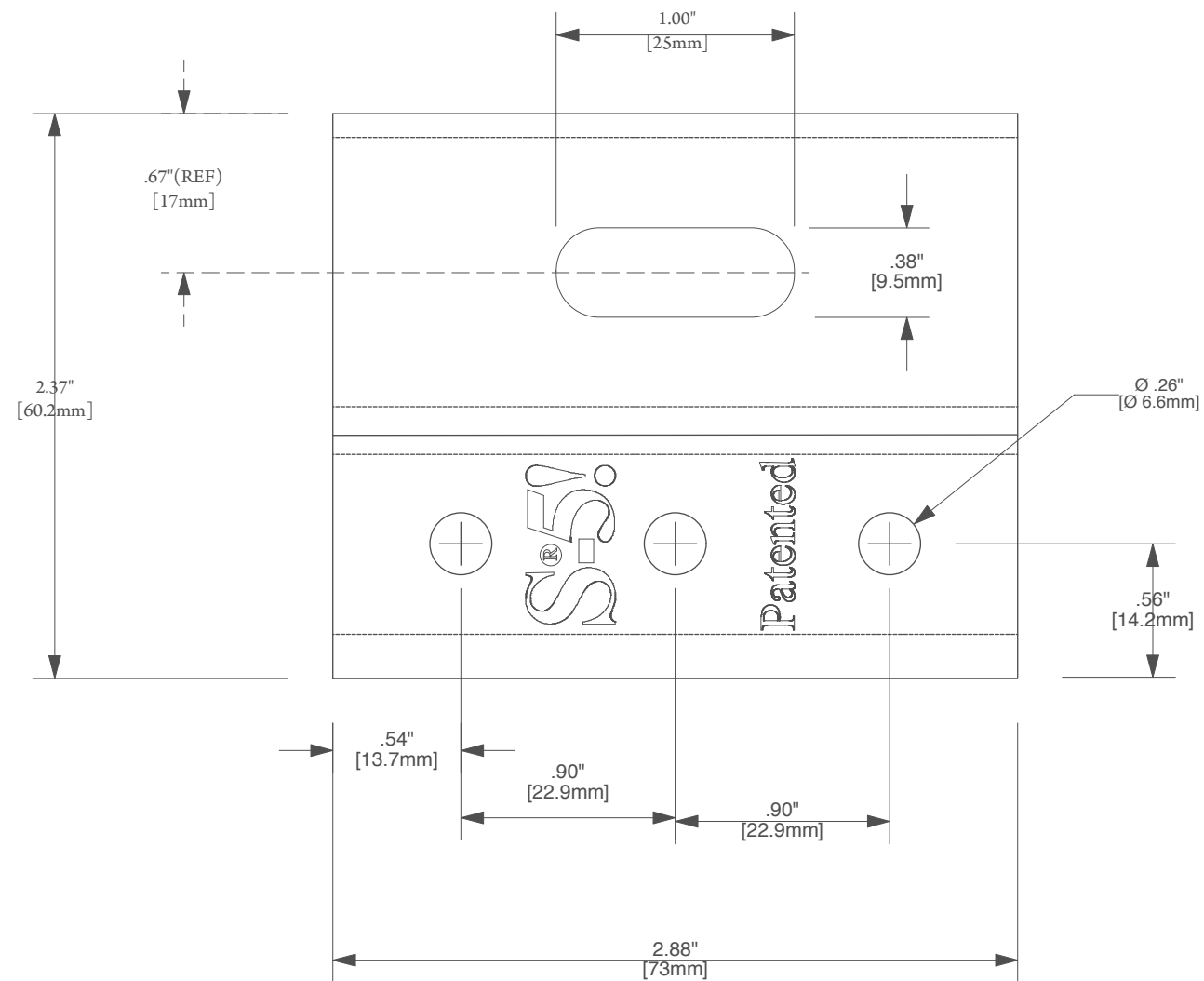
TOP VIEW
